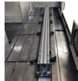
Complex medium-sized work pieces produced on a Haas CNC Vertical Machining Center (150" x 50" x 50")
